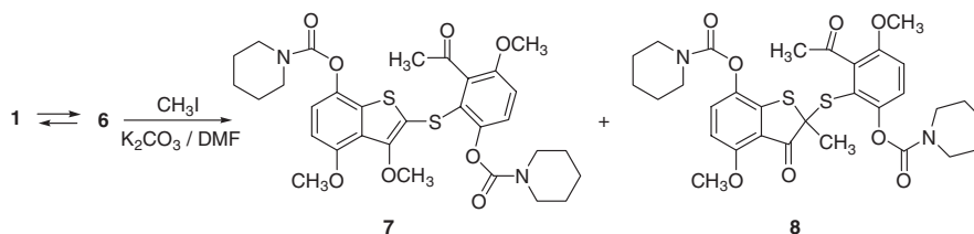
Scheme 3. Methylation of the spiro compound 1 .
