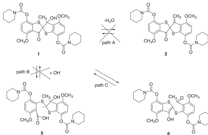
Scheme 2. The considered ways of isomerization of the spiro compound 1 .
