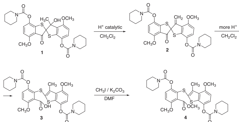
Scheme 1. Acid-induced transformations of the spiro compound 1 .
