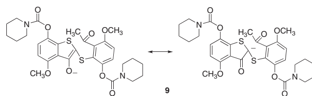
Figure 2. Mesomeric forms of anion 9 .
