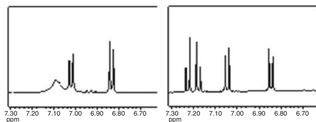
Figure 1. Influence of TFA on the shape of the aromatic protons peaks in ^1\text{H} NMR of 3 : \text{DMSO-}d_6 (left), \text{DMSO-}d_6 + 1 drop TFA (right) (To view the original spectra, see Supporting Information, part 1, pages 11–15).
